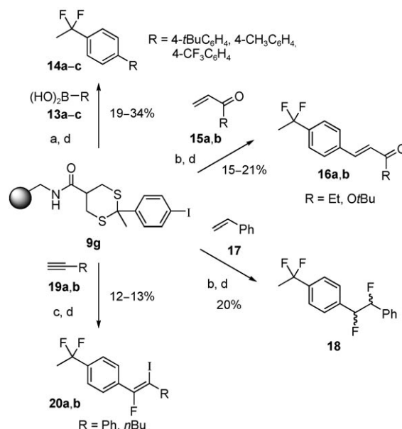
Scheme 4. Palladium-catalyzed cross-coupling reactions and subsequent cleavage: a) 13 , [\text{Pd}(\text{PPh}_3)_4] , \text{K}_3\text{PO}_4 , DMF, 100 °C, 2 d; b) 15 or 17 , \text{Pd}(\text{OAc})_2 , \text{PPh}_3 , \text{Et}_3\text{N} , DMF, 100 °C, 2 d; c) 19 , [\text{Pd}(\text{PPh}_3)_4] , \text{CuI} , \text{Et}_3\text{N} , DMF, 80 °C, 2 d; d) NIS, HF/py, -78 \rightarrow 0^\circ\text{C} , 3 h (yields over 4 steps).
