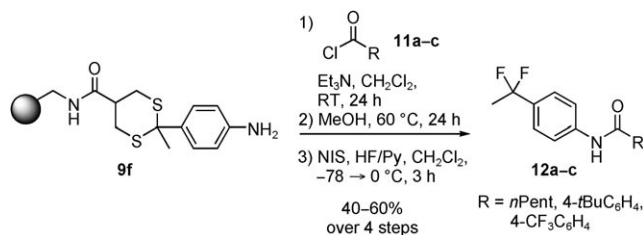
Scheme 3. Amide coupling and subsequent fluorinating cleavage.
