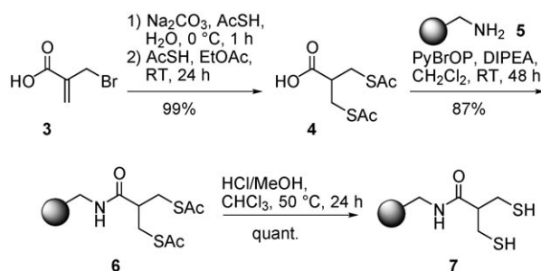
Scheme 1. Synthesis of the dithiol linker 7 starting from 2-(bromomethyl)acrylic acid ( 3 ).
