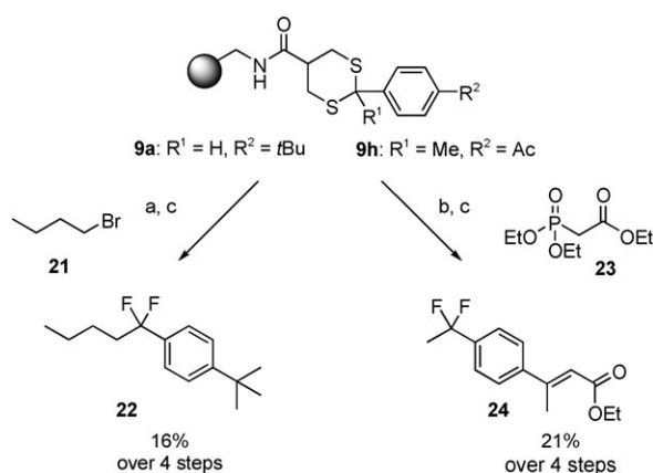
Scheme 5. Umpolung on the dithiane linker and HWE reaction followed by fluorinating cleavage: a) 9a , n BuLi, THF, -50 \rightarrow -20^\circ\text{C} , 4 h, then 21 , -50^\circ\text{C} \rightarrow \text{RT} , 15 h; b) 9h , 23 , KHMDS, [18]crown-6, THF, -78 \rightarrow 40^\circ\text{C} , 15 h; c) NIS, HF/py, -78 \rightarrow 0^\circ\text{C} , 3 h.
