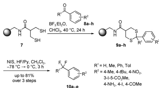
Scheme 2. Attachment of various aldehydes and ketones to a solid support and subsequent cleavage to give gem -difluoro compounds.
